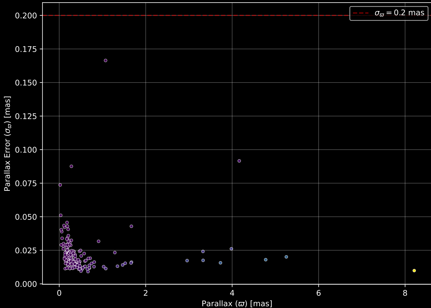
APOGEE DR17 Field: [113-04] Parallax Quality (n= 176)
