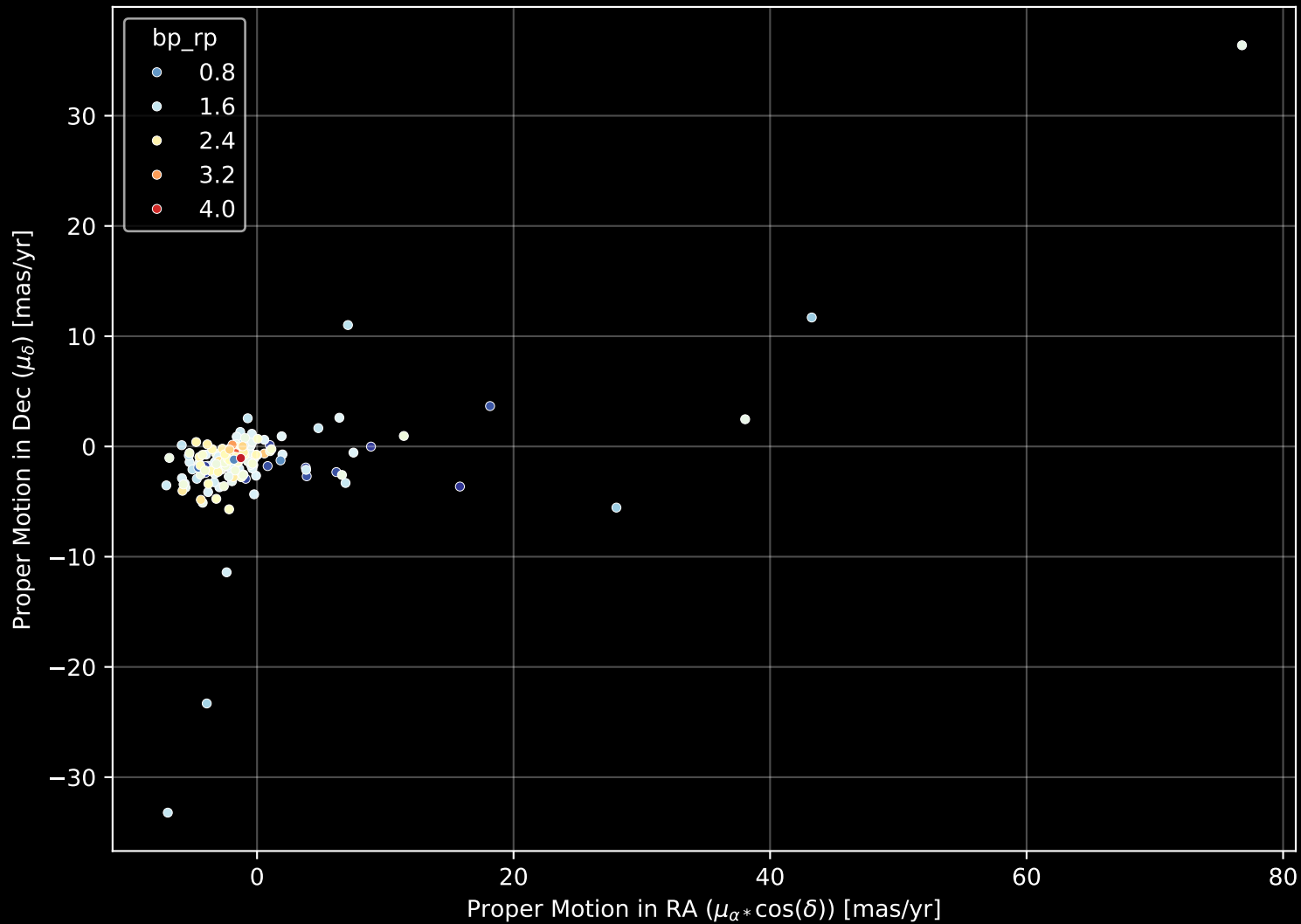
APOGEE DR17 Field: [113-04] Proper Motion Diagram (n= 176)
