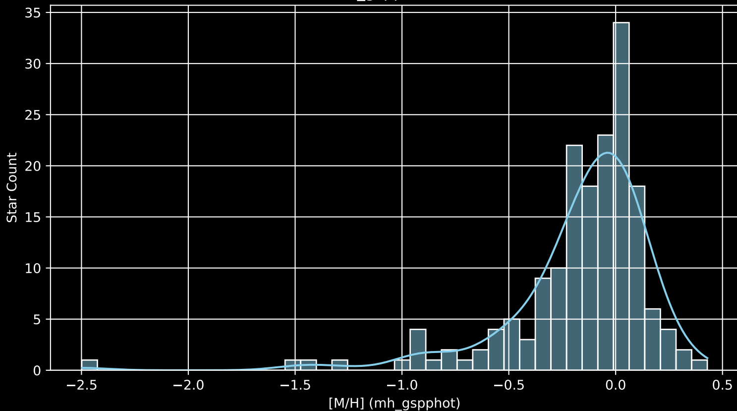
APOGEE DR17 Field: [113-04 [M/H] (mh_gspphot) (n= 174)
