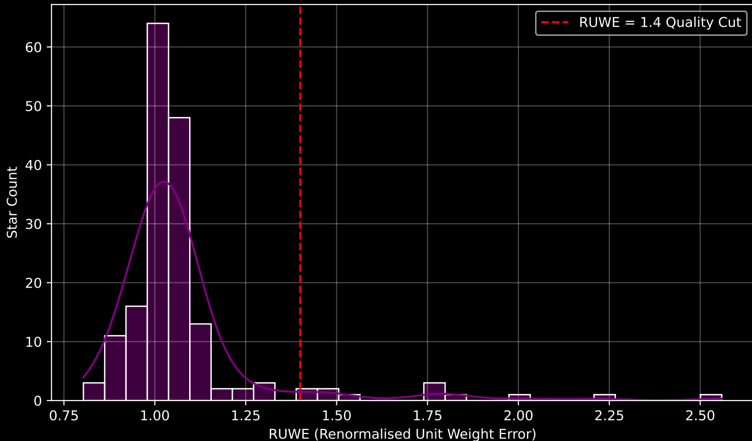
GAPOGEE DR17 Field [113-04] RUWE Distribution (n= 174)
