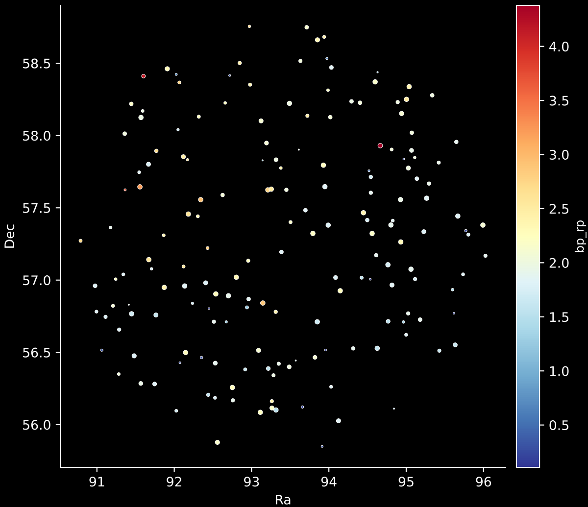
APOGEE DR17 Field: [113-04] Stars: 176
